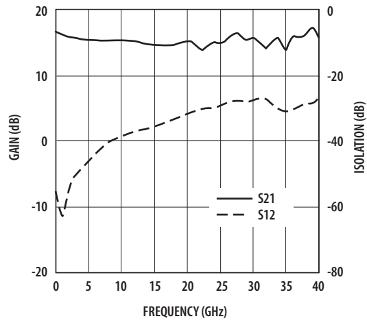
Figure 6. Gain and Reverse Isolation.
