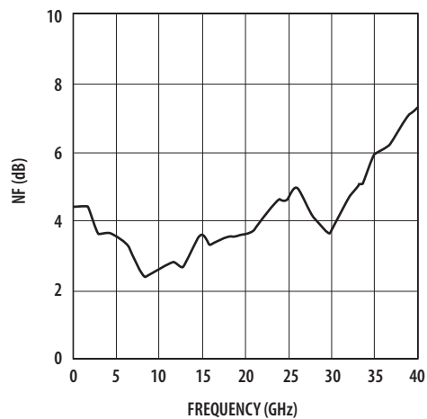
Figure 10. Noise Figure.
