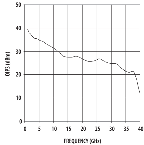
Figure 4. Output IP3.
