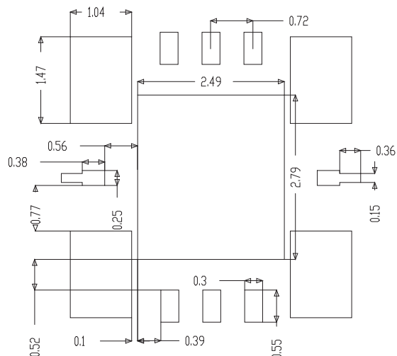
Figure 19. Stencil Outline Drawing (mm)
