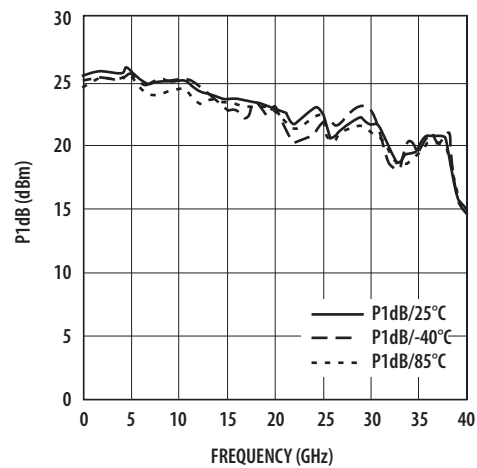
Figure 16. P1dB and Temperature.
