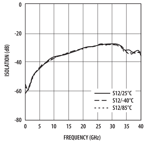
Figure 12. Isolation and Temperature.
