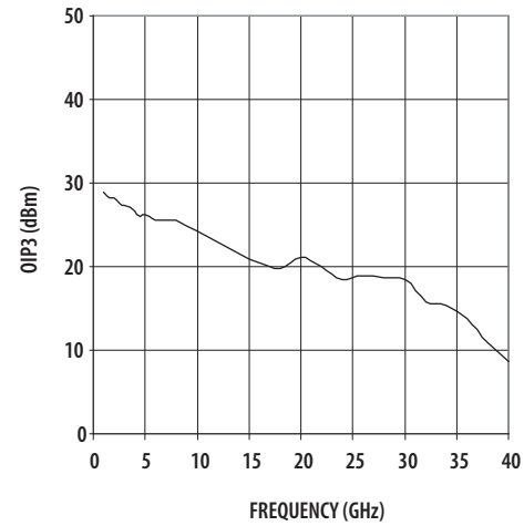
Figure 9. Output IP3.
