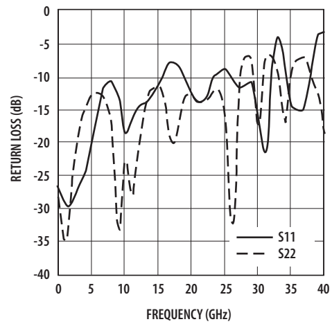
Figure 7. Return Loss (Input and Output).
