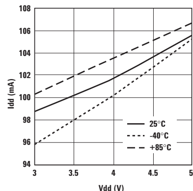
Figure 12. Bias Current Over Temperature.
