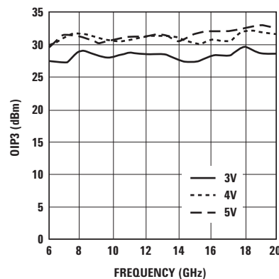
Figure 18. OIP3 Over Vdd.
