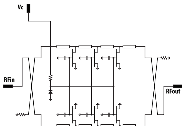
Figure16. Simplified schematic
