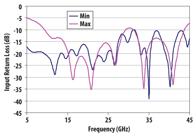
Figure 10. Output Return Loss vs Frequency at Min Attenuation
