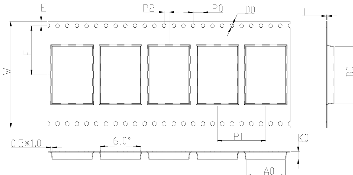
Figure 7 - Tape Specifications
