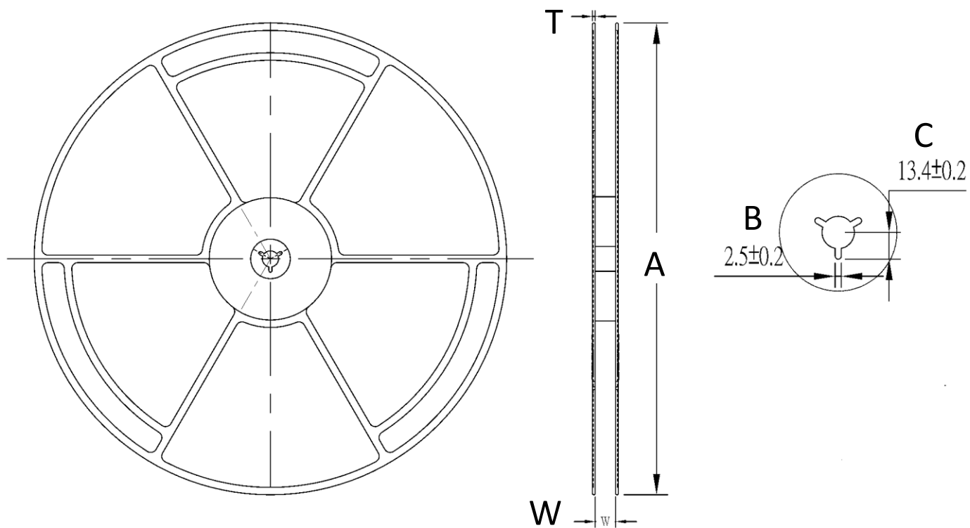
Figure 8 - Reel Specifications
