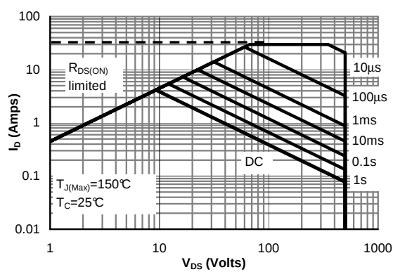
Figure 10: Maximum Forward Biased Safe Operating Area for AOTF9N50 (Note F)
