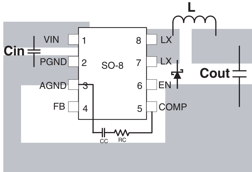
Figure 3. AOZ1017A PCB Layout
