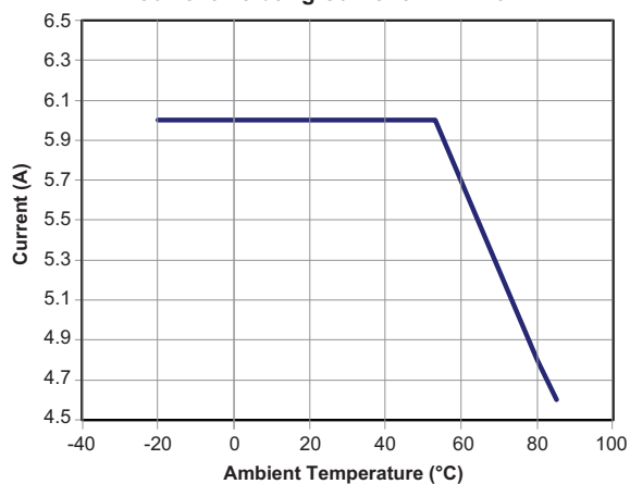
Current Derating Curve for DFN-10 4x4
