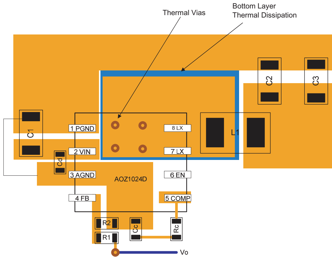
Figure 3. AOZ1024D (DFN 5x4) PCB Layout
