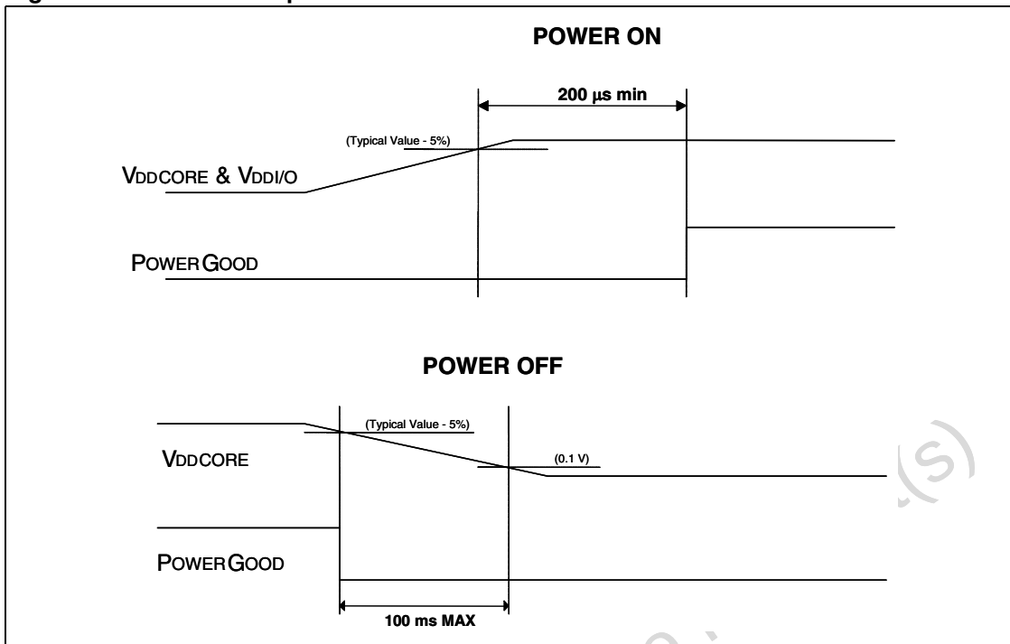
Figure 28. P_{\text{POWERGOOD}} requirement
