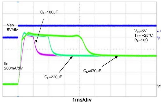
Inrush Current
