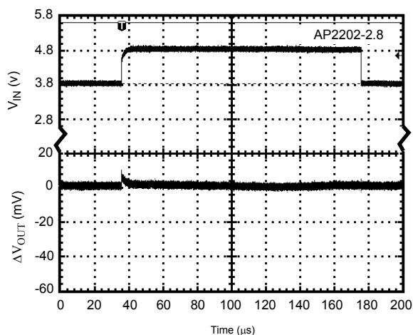
Figure 13. Line Transient (Conditions: V_{IN}=3.8V to 4.8V , V_{EN}=2V , I_{OUT}=100μA , C_{BYP}=100pF , C_{OUT}=10μF )
