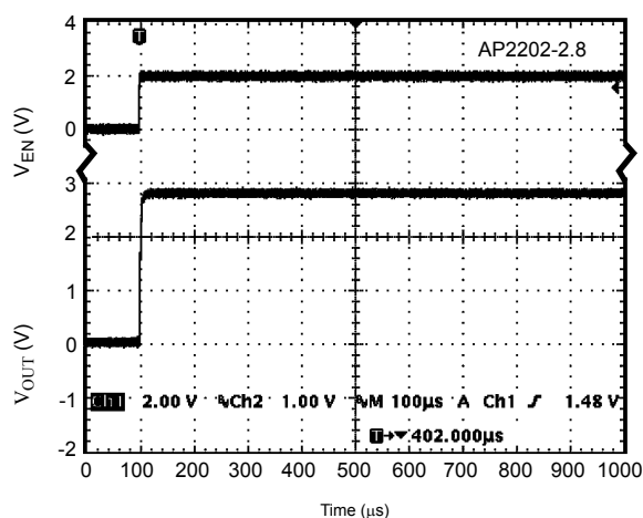
Figure 14. V_{EN}(on) vs. V_{OUT} (Conditions: V_{EN}=0V to 2V , V_{IN}=3.8V , I_{OUT}=30mA , C_{BYP}=open , C_{IN}=1.0μF , C_{OUT}=2.2μF )
