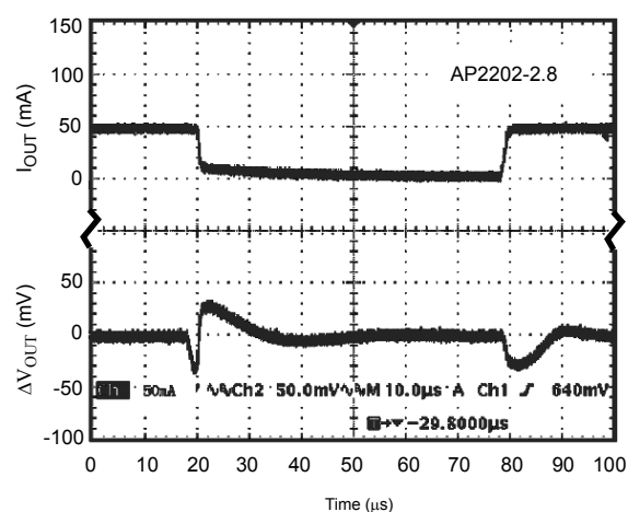
Figure 12. Load Transient (Conditions: V_{IN}=3.8V , C_{BYP}=100pF , V_{EN}=2V , I_{OUT}=5mA to 50mA , C_{IN}=1.0μF , C_{OUT}=2.2μF )
