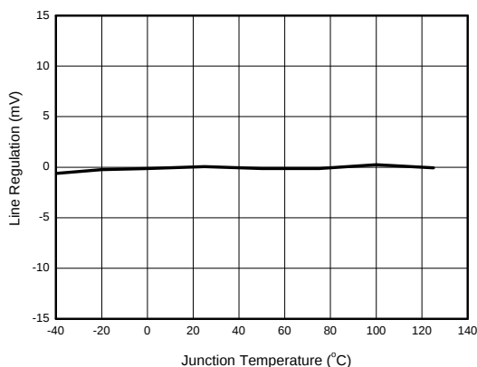
Figure 4. Line Regulation vs. Junction Temperature
