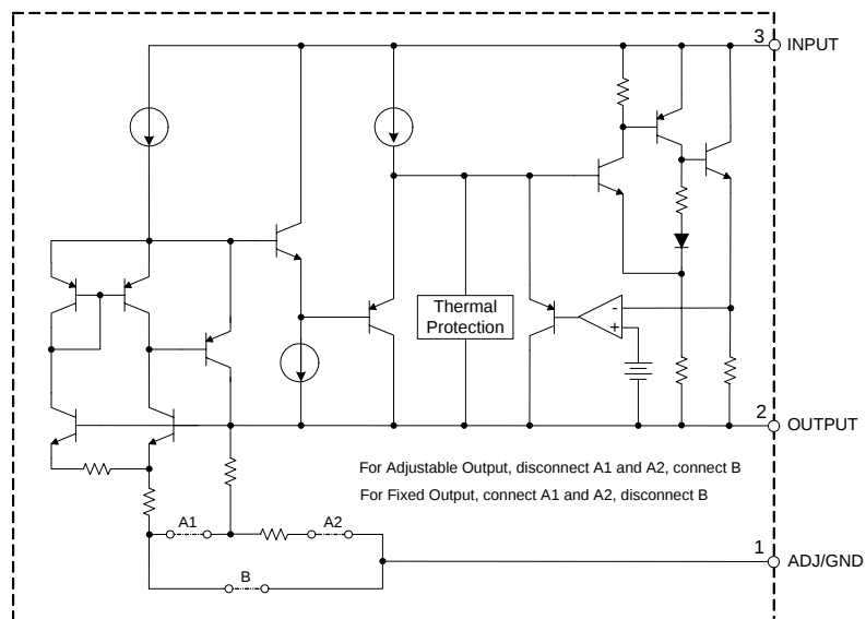
Figure 3. Functional Block Diagram of AP2317
