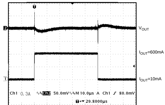
Figure 13. Load Transient Response
