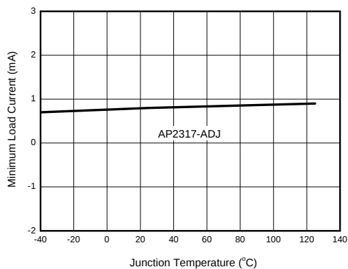
Figure 8. Minimum Load Current vs. Junction Temperature
