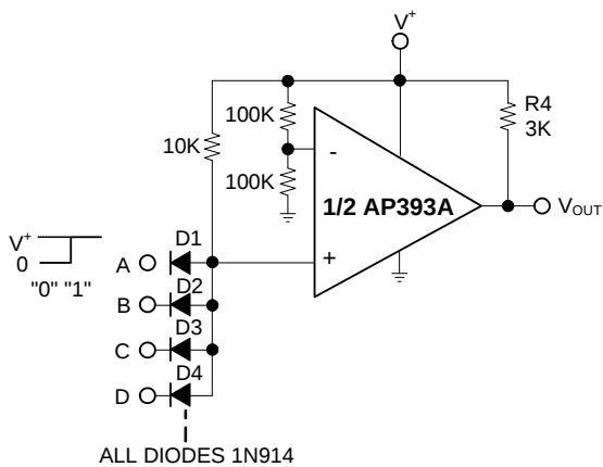
AND Gate
