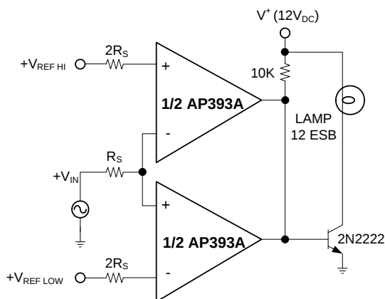
Limit Comparator
