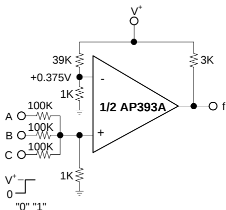
AND Gate
