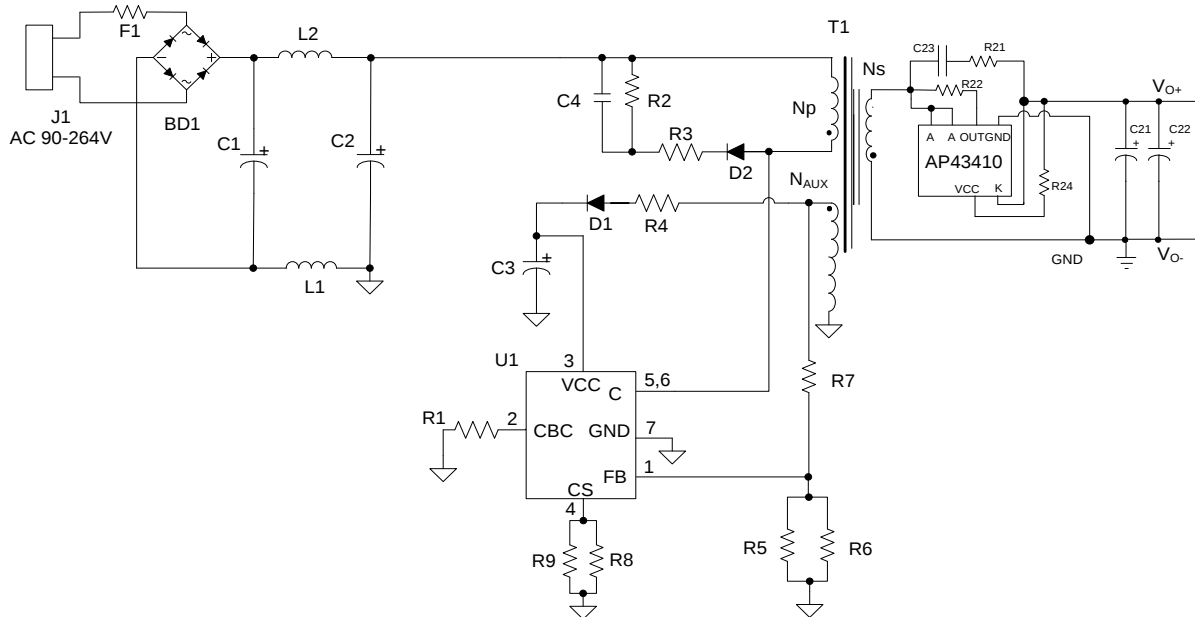
For AP3984+AP43410 (5V/1A)
