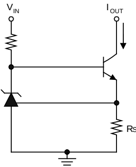
Fig. 7 Constant-Current Sink
