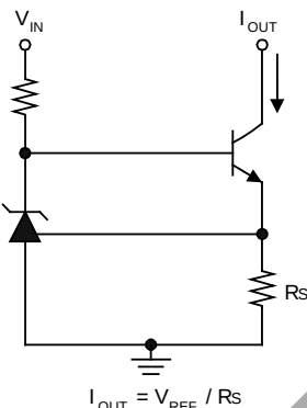
Fig. 7 Constant-Current Sink
