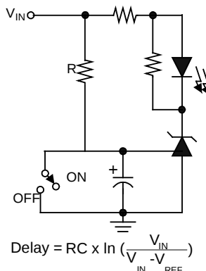
Fig. 5 Delay Timer
