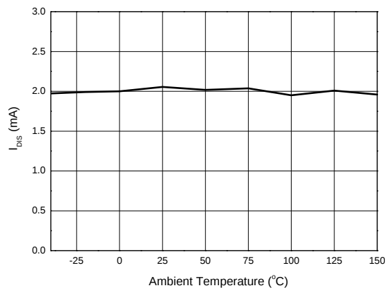
Discharge Current vs. Ambient Temperature
