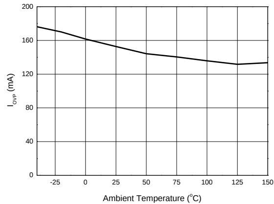
Overshoot Current for Discharge vs. Ambient Temperature
