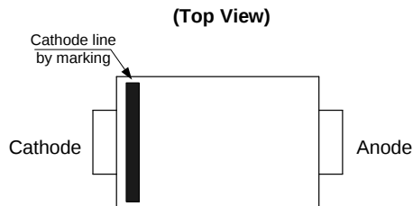
SOD-123
