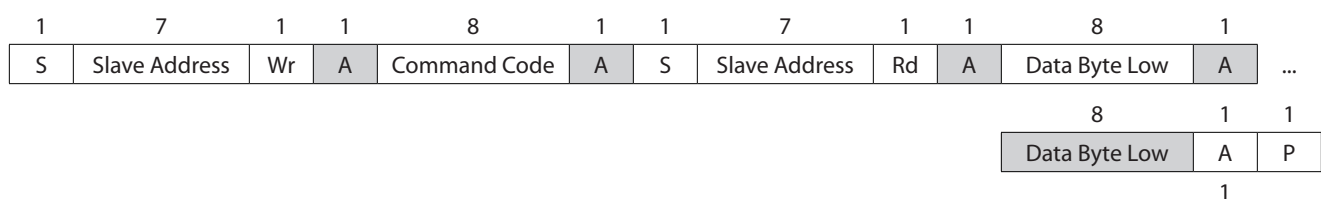
Figure 11. SMBus Read Word Protocol
