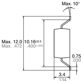
Surface mount terminal type
