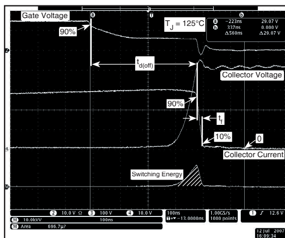
Figure 24, Turn-off Switching Waveforms and Definitions
