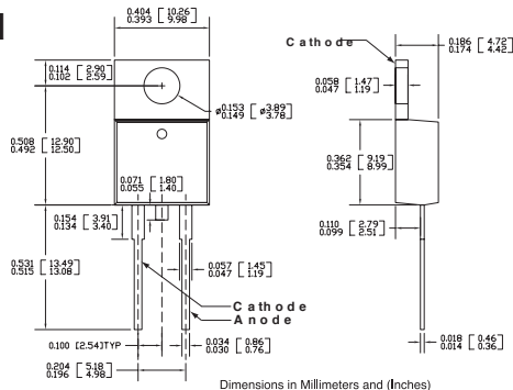
TO-220 2-Lead
