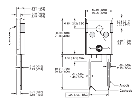
TO-247 2-Lead
