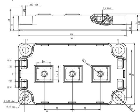
SP6 - 3 outputs
