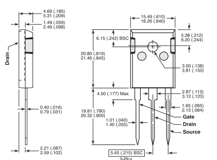
TO-247 3-Lead
