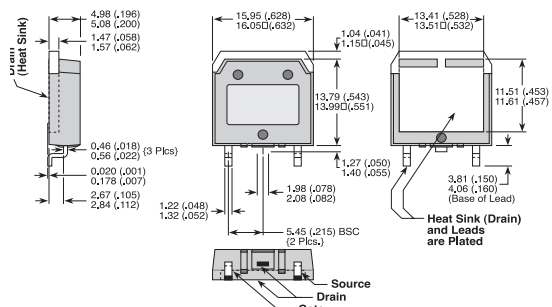
D 3 Pak or TO-268
