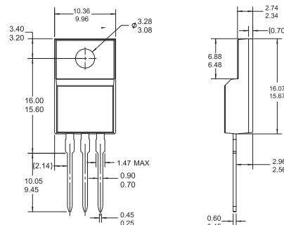
TO-220 [KF]
