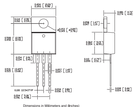
TO-220 3-Lead
