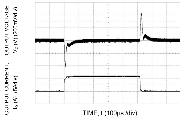
Figure 28. Transient Response to Dynamic Load Change from 0% 50% to 0%.
