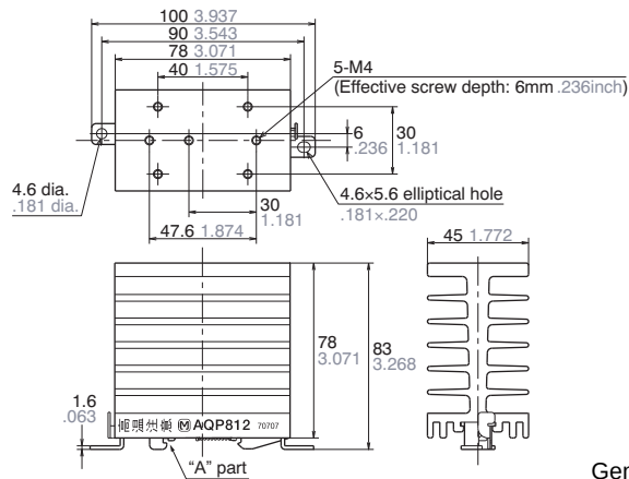
External dimensions
