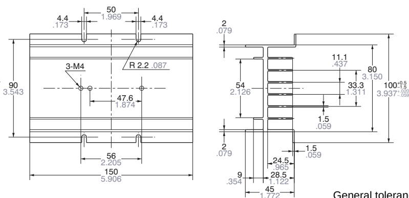
External dimensions
