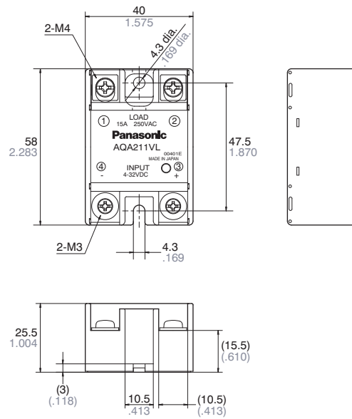
External dimensions
