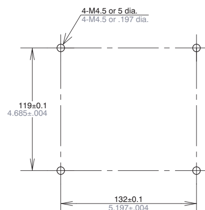
Mounting dimensions
