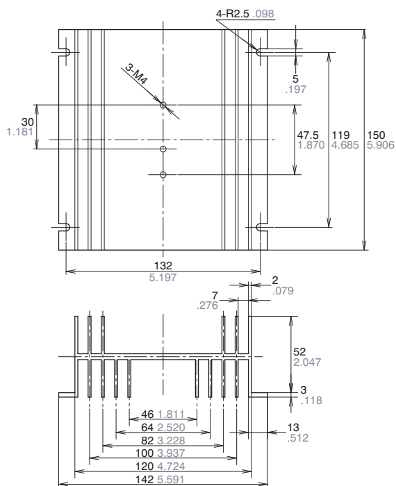
External dimensions
