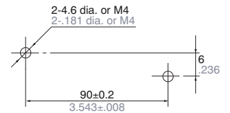
Mounting dimensions
