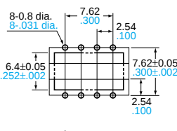
Mounting pad (Top view)
