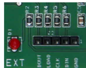
Figure 5: External interface
