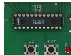
Figure 3: Mounted Chip
