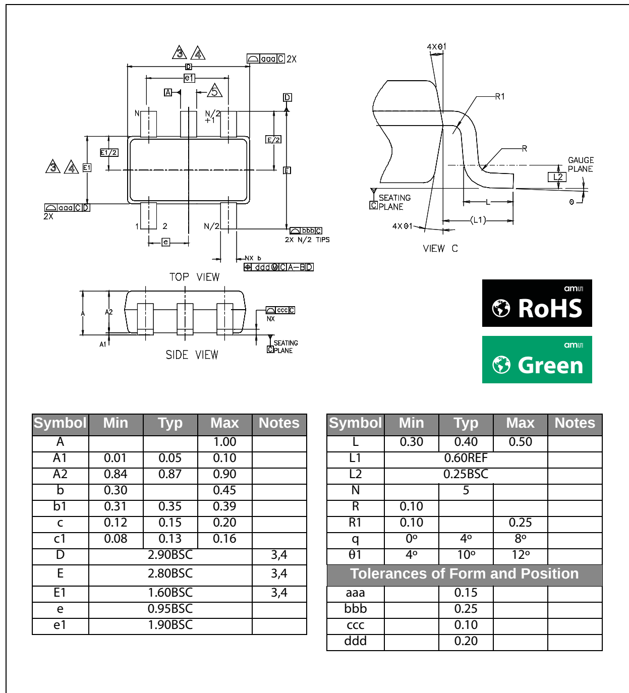
Figure 26: TSOT23-5 Package
