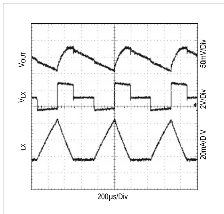
Figure 22: Switching Waveform; V_{OUT} = 3.0V
