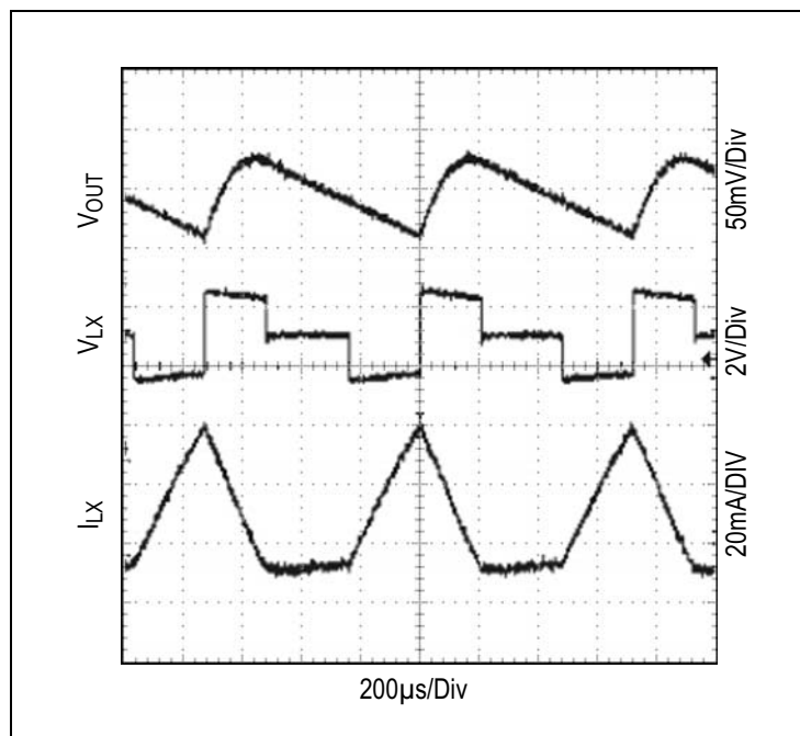
Figure 22: Switching Waveform; V_{OUT} = 3.0V
