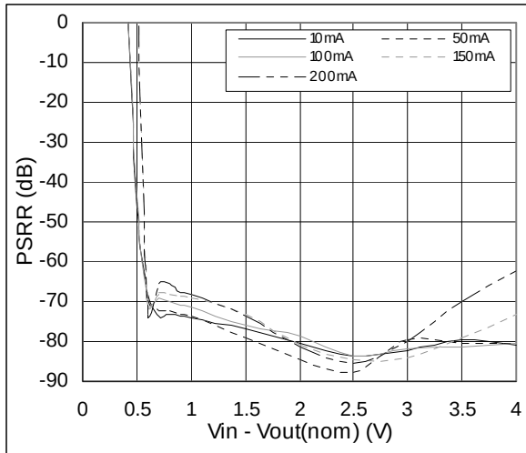
Figure 29. PSRR vs. V_{IN}-V_{OUT(NOM)} , V_{OUT}=1.5V
