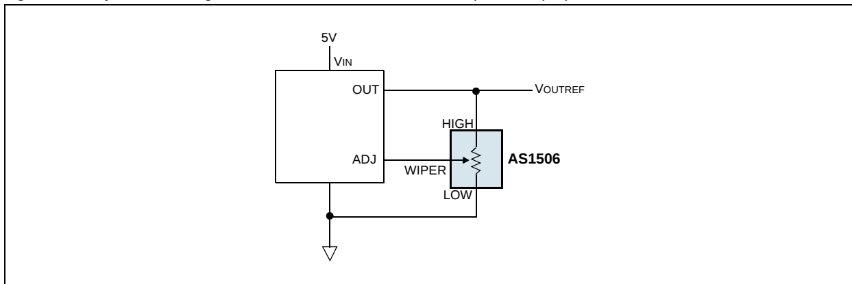
Figure 28. Adjustable Voltage Reference Circuit – V_{OUT} = 1.23V(50k\Omega/R_2(k\Omega))
