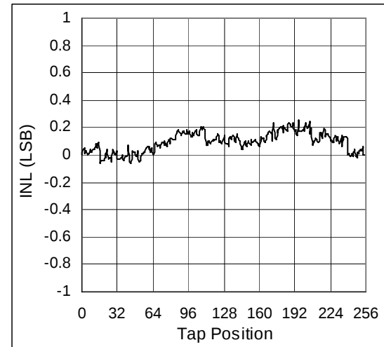
Figure 14. INL vs. TAP Position 100k \Omega , Varistor
