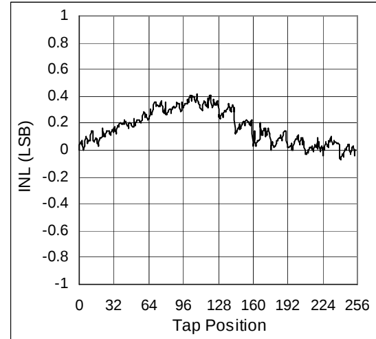
Figure 14. INL vs. TAP Position 100k \Omega , Varistor
