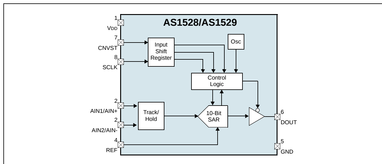
Figure 1. Block Diagram
