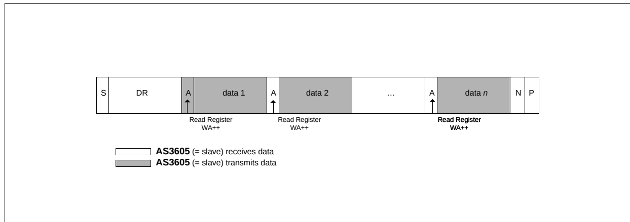
Figure 24. I 2 C Current Address Read
