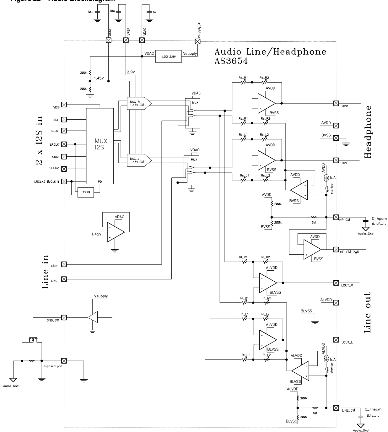
Figure 22 – Audio Blockdiagram
