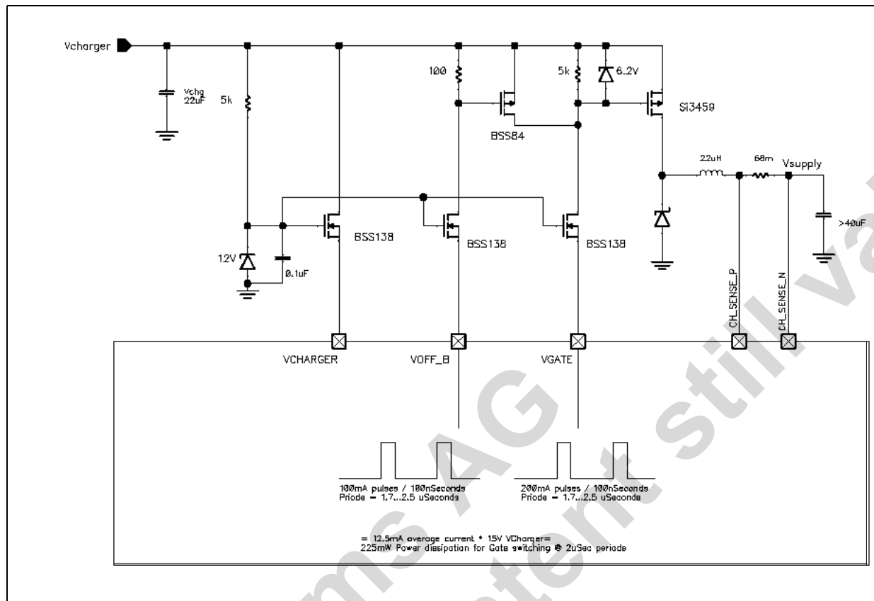
Figure 15. Charger Block Diagram for voltages >15V (Protection up to 50V; minimum V charger voltage 8V)
