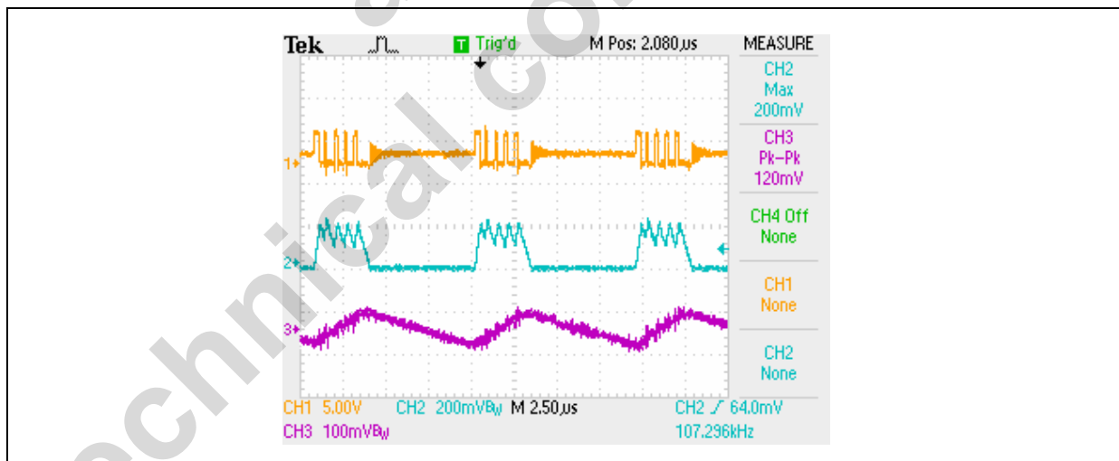
Figure 29. sdX_dis_curmin=0 operation
