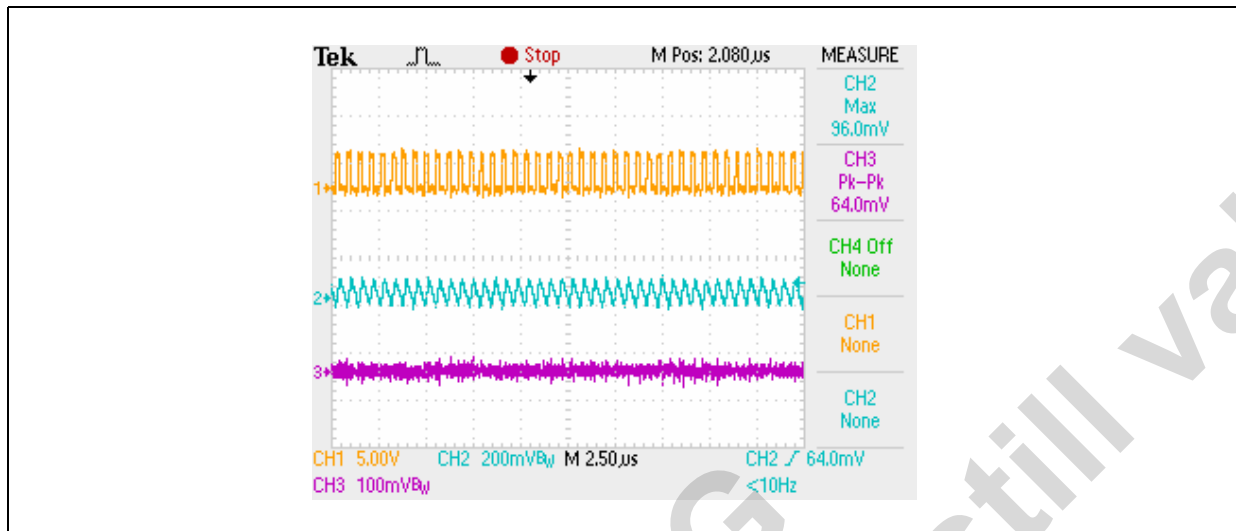
Figure 28. sdX_dis_curmin=1 operation
