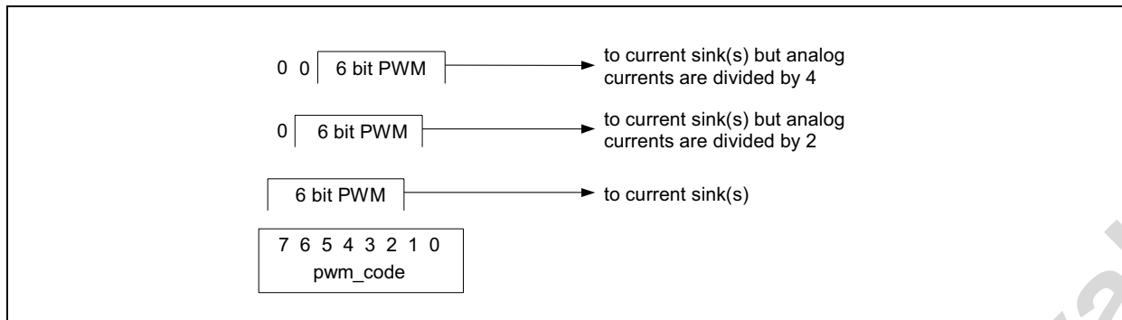
Figure 21. PWM Control
