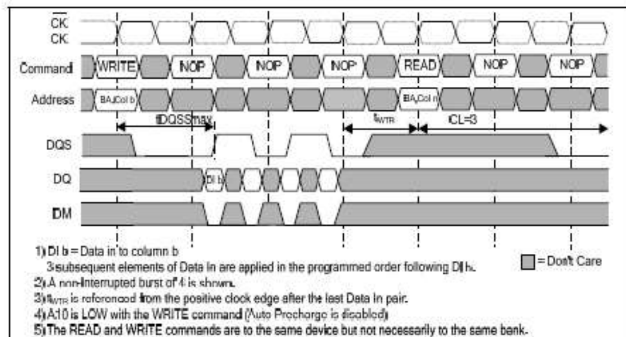
Figure 28 — Non-Interrupting Write to Read
