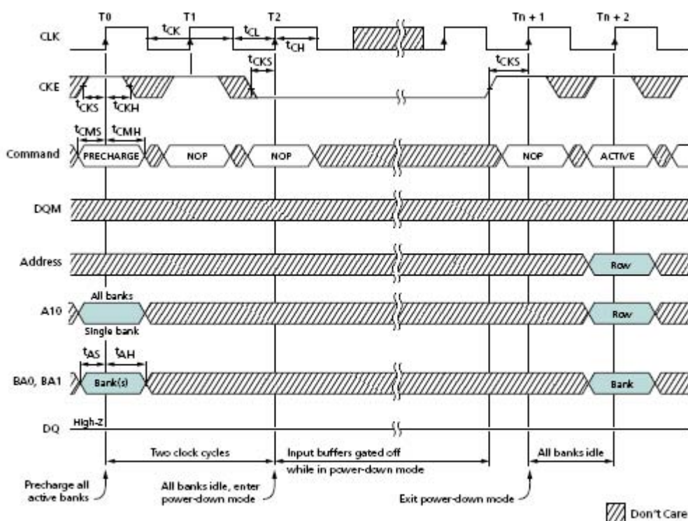
Figure 47: Power-Down Mode
