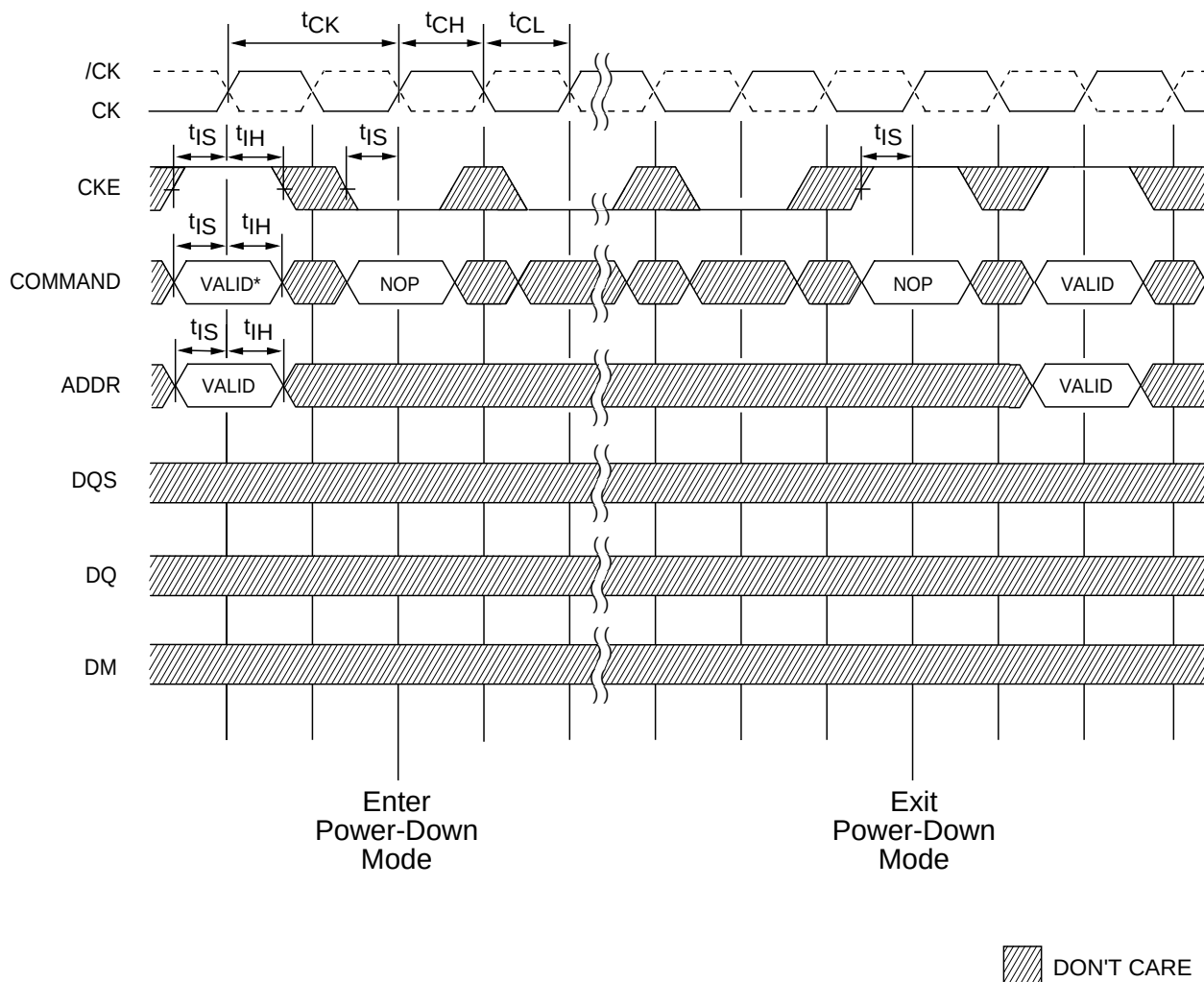
Figure 39 - POWER-DOWN MODE
