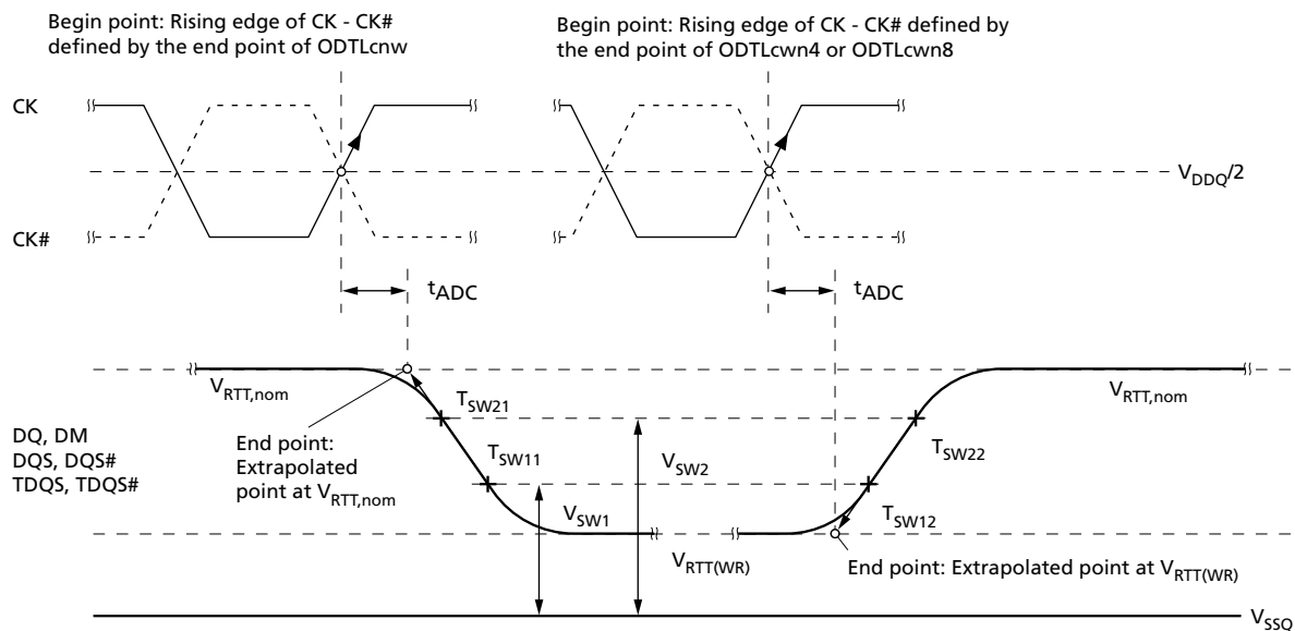
Figure 23: t_{ADC} Definition
