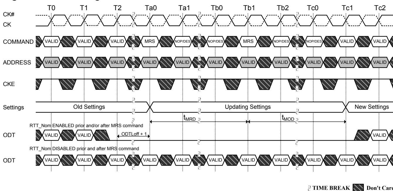
Figure 6. t_{MRD} timing
