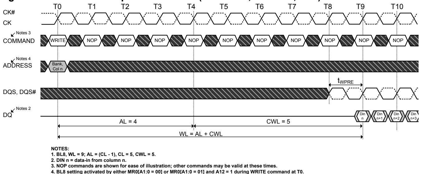
Figure 42. WRITE Burst Operation WL = 9 (AL = CL-1, CWL = 5, BL8)
