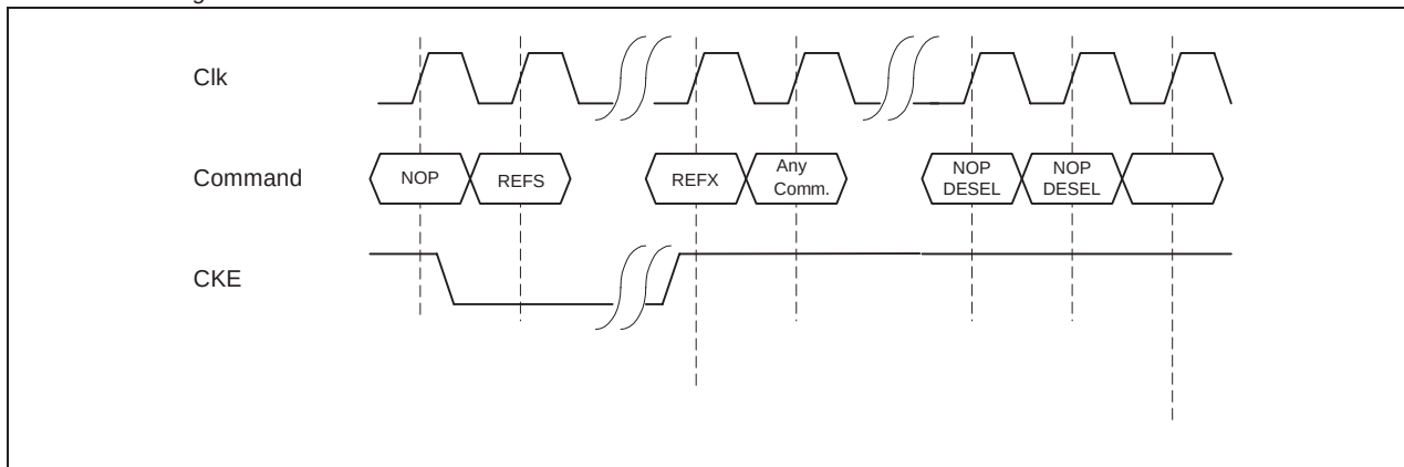
Self Refresh timing
