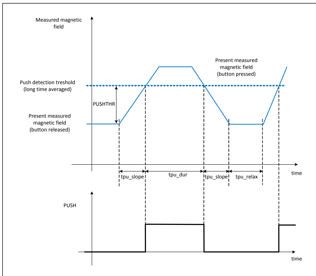
Figure 27: Pushbutton Detection Function
