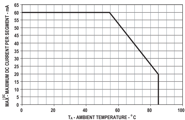
Figure 5. Forward Current versus Ambient Temperature derated based on T_j = 110^\circ\text{C} and thermal resistance at 400^\circ\text{C/W}
