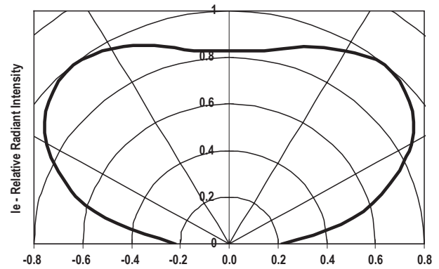
Figure 4. Angular Displacement Vs Relative Radiant Intensity
