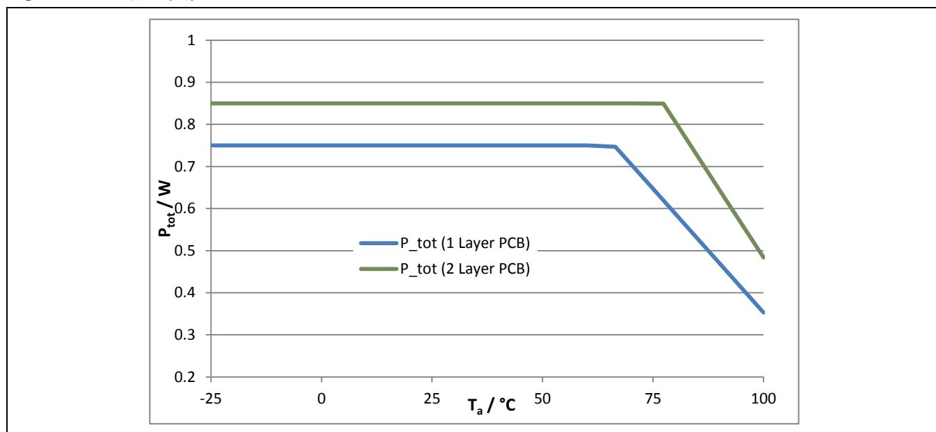
Figure 2.1 P_{tot} = f(T_a)
