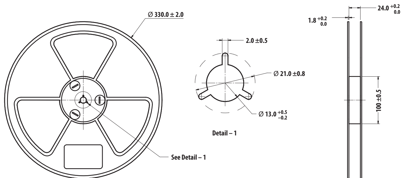
Figure 32. Reel dimensions.
