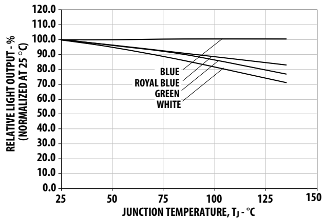
Figure 20. Relative Light Output vs. Junction Temperature.
