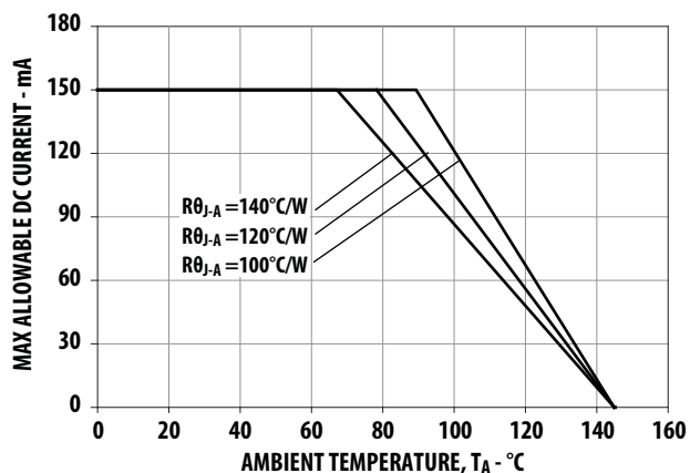
Figure 7. Maximum forward current vs. ambient temperature. Derated based on T_{JMAX} = 145^\circ\text{C} , R_{\theta JA} = 100^\circ\text{C/W} , 120^\circ\text{C/W} and 140^\circ\text{C/W}
