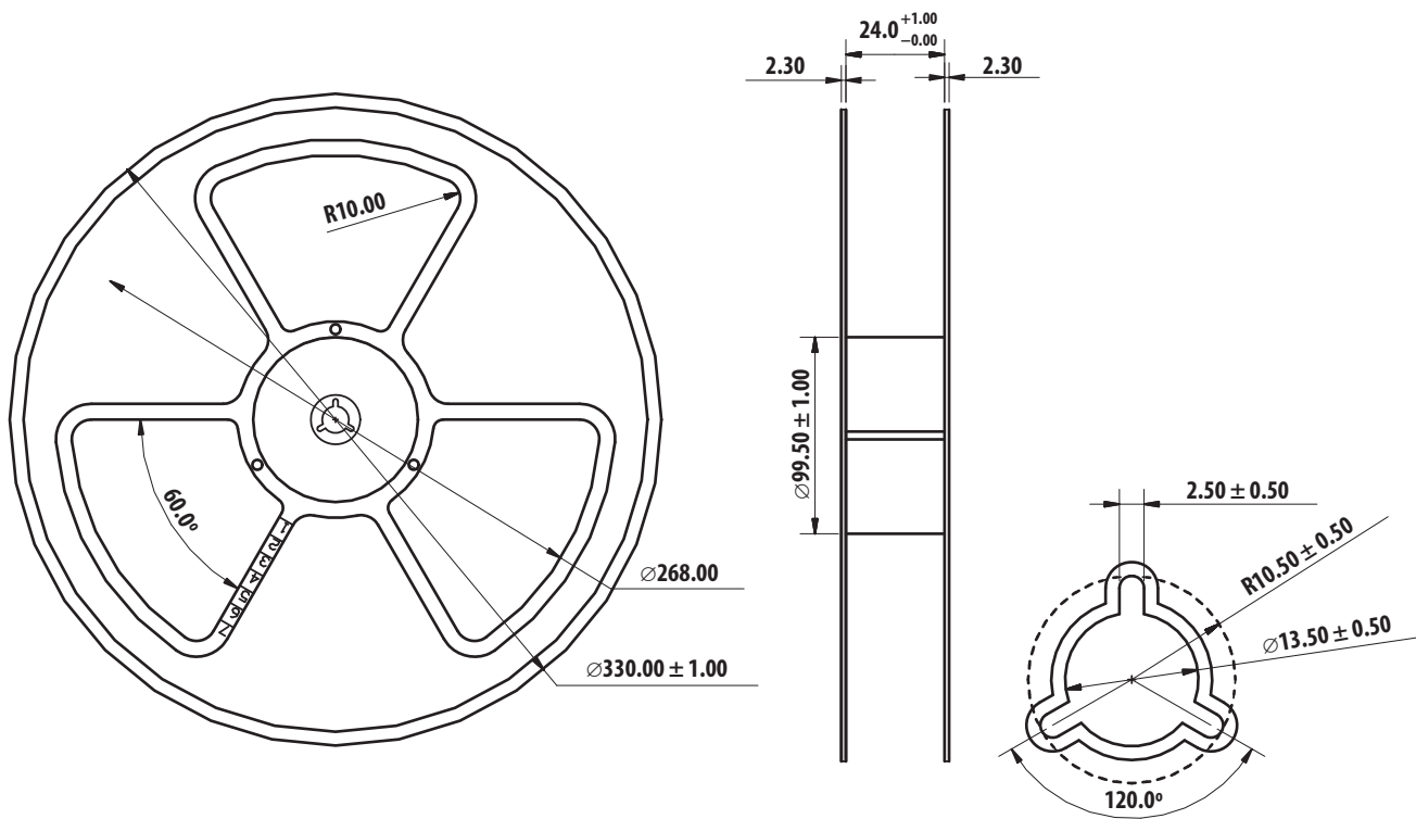
Figure 16. Reel dimensions
