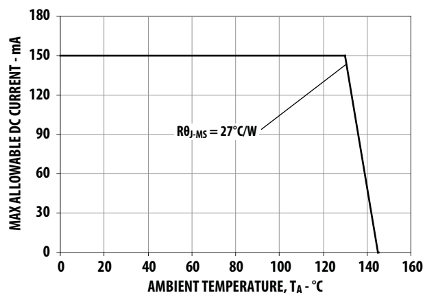
Figure 8. Maximum Forward Current vs. Metal Slug Temperature. Derated based on T_{JMAX} = 145^\circ\text{C} , R_{\theta JS} = 27^\circ\text{C/W} .
