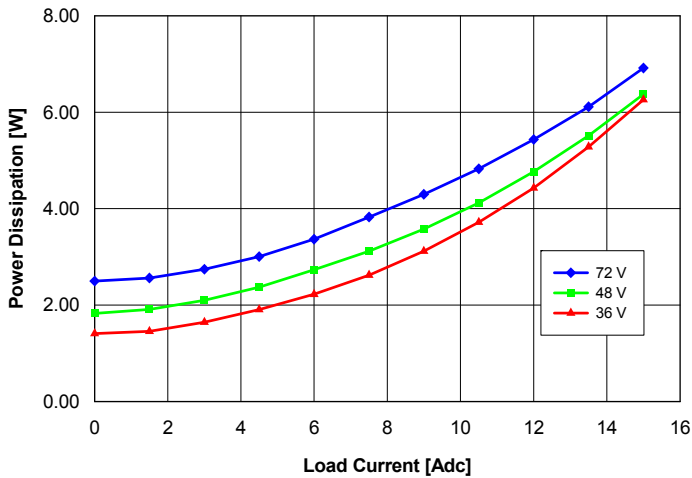
Fig. 15: Power dissipation vs. load current and input voltage for converter mounted vertically with air flowing from pin 3 to pin 1 at a rate of 300 LFM (1.5 m/s) and T_a = 25^\circ\text{C} .
