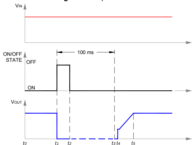
Fig. 8: Start-up scenario #3.
