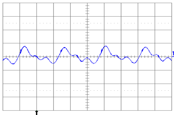
Fig. 21: Output voltage ripple (20 mV/div.) at full rated load current into a resistive load with C_o = 10 \mu\text{F} tantalum + 1\mu\text{F} ceramic and V_{in} = 48 \text{ V} . Time scale: 1 \mu\text{s}/\text{div} .
