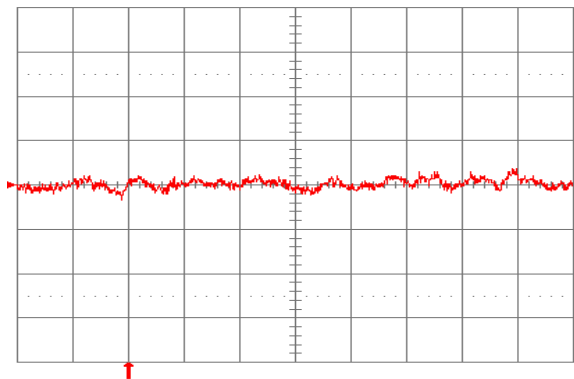
Fig. 24: Input reflected ripple current, i_s (10 mA/div), measured through 10 \mu\text{H} at the source at full rated load current and V_{in} = 48 \text{ V} . Refer to Fig. 22 for test setup. Time scale: 1 \mu\text{s}/\text{div} .
