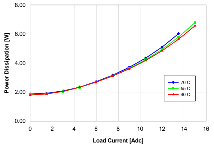
Fig. 16: Power dissipation vs. load current and ambient temperature for converter mounted vertically with V_{in} = 48\text{ V} and air flowing from pin 3 to pin 1 at a rate of 200 LFM (1.0 m/s).
