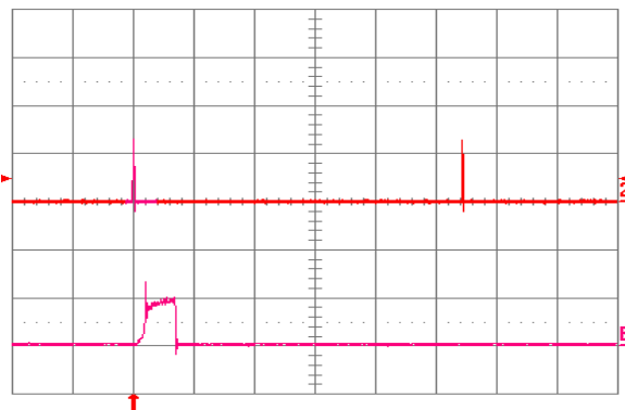
Fig. 26: Load current (top trace, 20 A/div, 20 ms/div) into a 10 mΩ short circuit during restart, at Vin = 48 V. Bottom trace (20 A/div, 1 ms/div) is an expansion of the on-time portion of the top trace.
