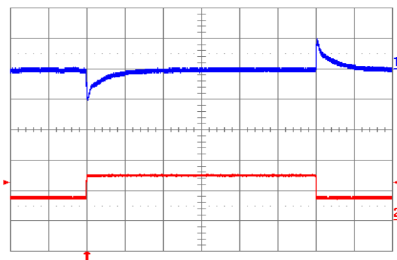
Fig. 20: Output voltage response to load current step-change (3.75 A – 7.5 A – 3.75 A) at V_{in} = 48\text{ V} . Top trace: output voltage (100 mV/div.). Bottom trace: load current (5 A/div.). Current slew rate: 5 A/ \mu\text{s} . C_o = 450\text{ }\mu\text{F} tantalum + 1 \mu\text{F} ceramic. Time scale: 0.2 ms/div.
