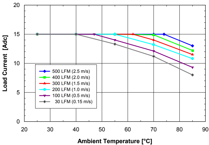
Fig. 11: Available load current vs. ambient temperature and airflow rates for ASQ48S15033 converter mounted vertically with V_{in} = 48 V, air flowing from pin 3 to pin 1 and maximum FET temperature \leq 120^{\circ}\text{C} .
