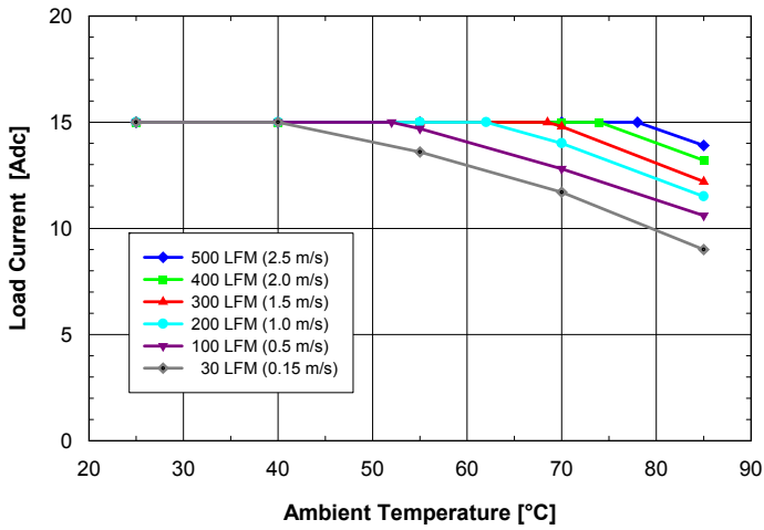
Fig. 9: Available load current vs. ambient air temperature and airflow rates for ASQ48T15033 converter with D height pins mounted vertically with V_{in} = 48 V, air flowing from pin 3 to pin 1 and maximum FET temperature \leq 120^{\circ}\text{C} .
