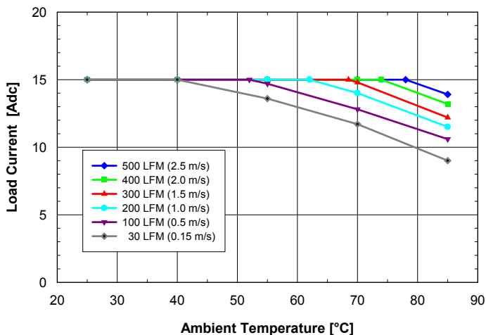
Fig. 1: Available load current vs. ambient air temperature and air-flow rates for ASQ48T15033 converter with D height pins mounted vertically with air flowing from pin 3 to pin 1, MOSFET temperature \leq 120^\circ\text{C} , V_{in} = 48\text{ V} .
