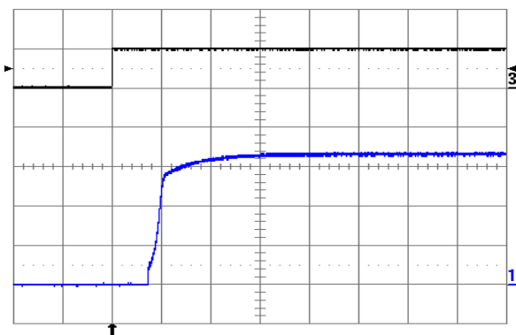
Fig. 17: Turn-on transient at full rated load current (resistive) with no output capacitor at V_{in} = 48\text{ V} , triggered via ON/OFF pin. Top trace: ON/OFF signal (5 V/div.). Bottom trace: output voltage (1 V/div.) Time scale: 2 ms/div.
