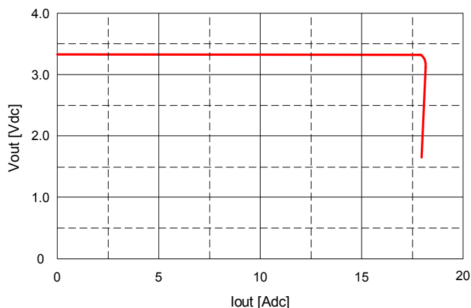
Fig. 25: Output voltage vs. load current showing current limit point and converter shutdown point. Input voltage has almost no effect on current limit characteristic.
