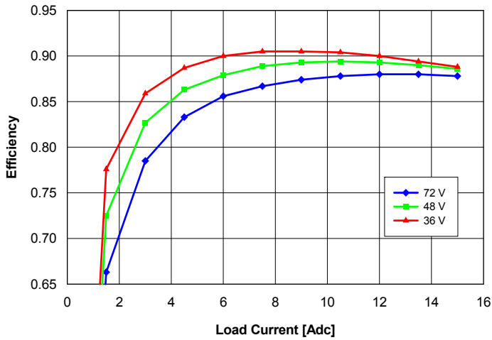
Fig. 13: Efficiency vs. load current and input voltage for converter mounted vertically with air flowing from pin 3 to pin 1 at a rate of 300 LFM (1.5 m/s) and T_a = 25^\circ\text{C} .
