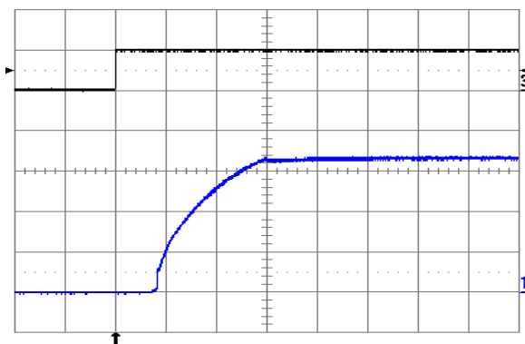
Fig. 18: Turn-on transient at full rated load current (resistive) plus 10,000 \mu\text{F} at V_{in} = 48\text{ V} , triggered via ON/OFF pin. Top trace: ON/OFF signal (5 V/div.). Bottom trace: output voltage (1 V/div.). Time scale: 2 ms/div.
