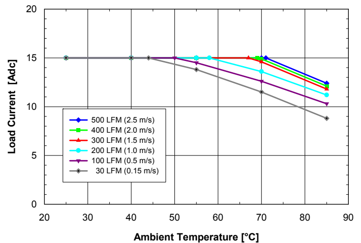
Fig. 12: Available load current vs. ambient temperature and airflow rates for ASQ48S15033 converter mounted horizontally with V_{in} = 48 V, air flowing from pin 3 to pin 1 and maximum FET temperature \leq 120^{\circ}\text{C} .
