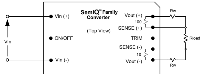
Fig. 3: Remote sense circuit configuration.
