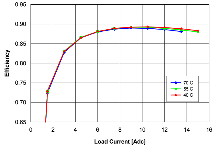
Fig. 14: Efficiency vs. load current and ambient temperature for converter mounted vertically with V_{in} = 48\text{ V} and air flowing from pin 3 to pin 1 at a rate of 200 LFM (1.0 m/s).
