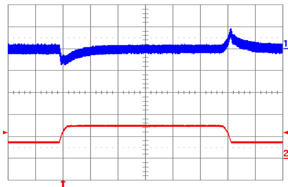
Fig. 19: Output voltage response to load current step-change (3.75 A – 7.5 A – 3.75 A) at V_{in} = 48\text{ V} . Top trace: output voltage (100 mV/div.). Bottom trace: load current (5 A/div.). Current slew rate: 0.1 A/ \mu\text{s} . C_o = 1\text{ }\mu\text{F} ceramic. Time scale: 0.2 ms/div.
