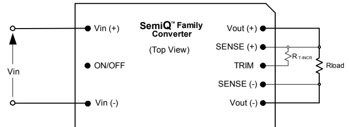
Fig. 4: Configuration for increasing output voltage.
