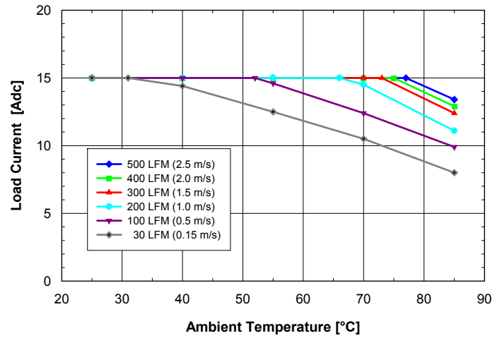
Fig. 10: Available load current vs. ambient air temperature and airflow rates for ASQ48T15033 converter with D height pins mounted horizontally with V_{in} = 48 V, air flowing from pin 3 to pin 1 and maximum FET temperature \leq 120^{\circ}\text{C} .
