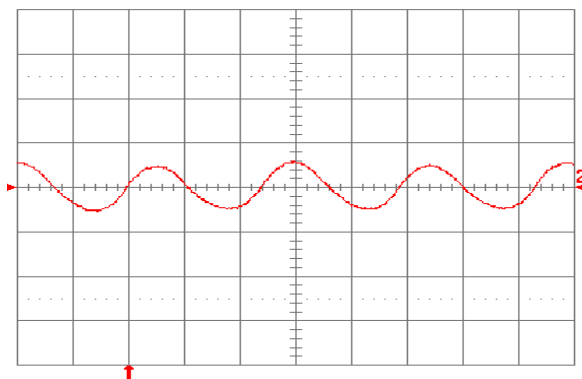
Fig. 23: Input reflected ripple current, i_c (100 mA/div), measured at input terminals at full rated load current and V_{in} = 48 \text{ V} . Refer to Fig. 22 for test setup. Time scale: 1 \mu\text{s}/\text{div} .
