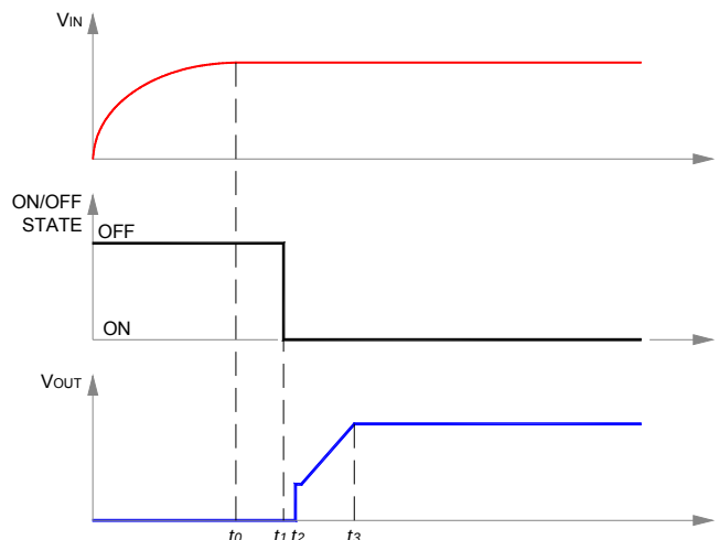
Fig. 7: Start-up scenario #2.
