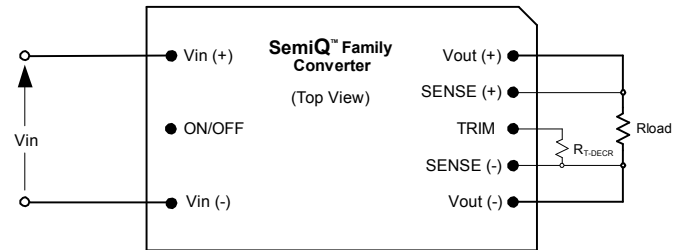
Fig. 5: Configuration for decreasing output voltage.
