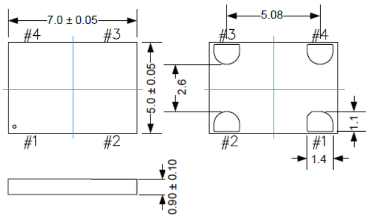
7.0 x 5.0mm Package (Option "V")
