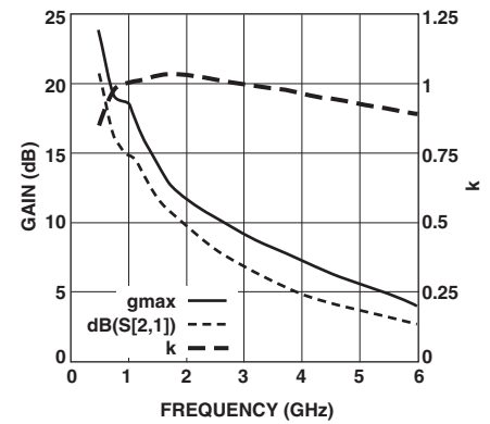
Figure 15. Gain vs. Frequency at 5 V, 10 mA.
