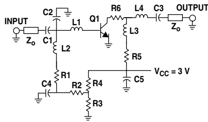
Figure 16. Schematic Diagram.
