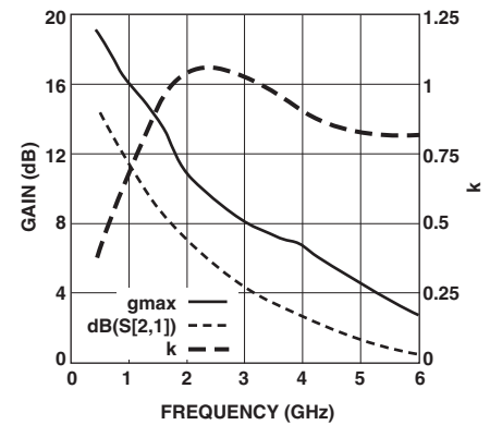
Figure 10. Gain vs. Frequency at 2.7 V, 2 mA.
