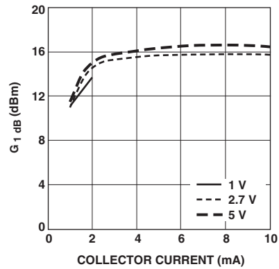
Figure 8a. G1dB vs. Collector Current and Voltage (at 900MHz).
