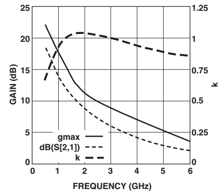
Figure 11. Gain vs. Frequency at 2.7 V, 5 mA.
