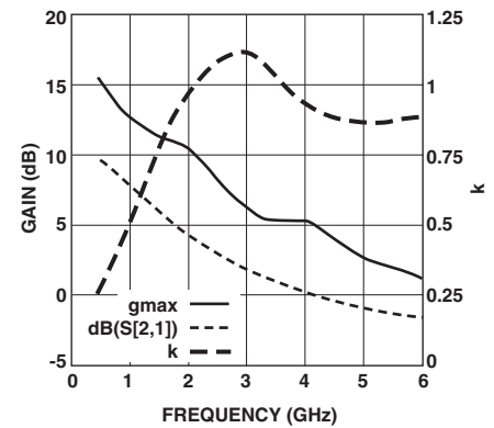
Figure 9. Gain vs. Frequency at 1 V, 1 mA.
