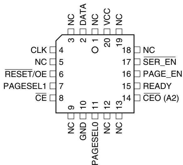
20-lead PLCC
